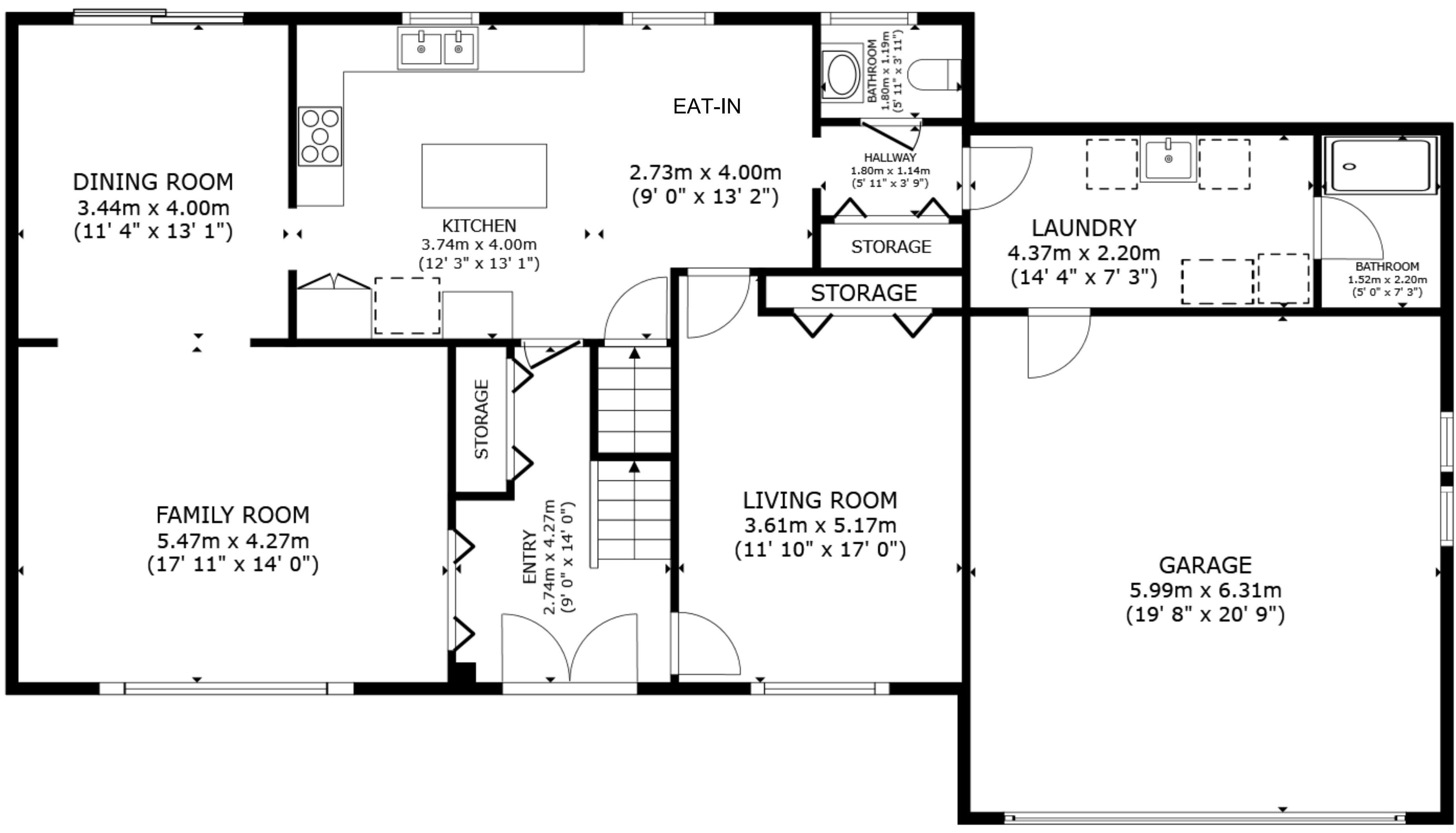
FLOOR 2
